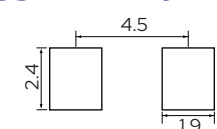
Top View Suggested Layout
